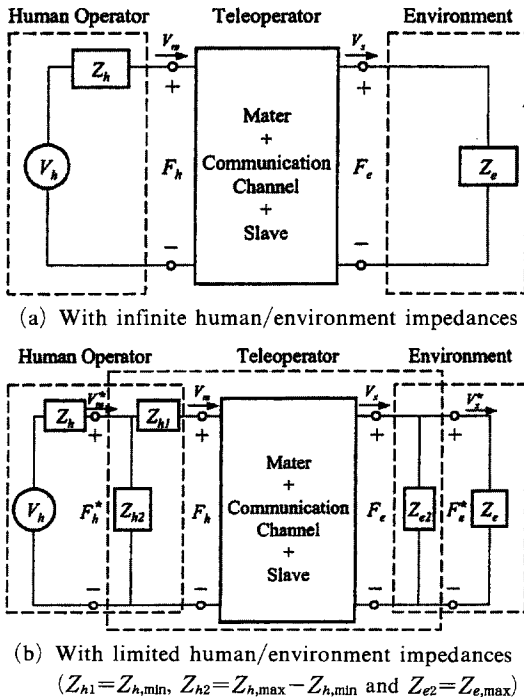
Fig. 3 A two-port model of teleoperation systems ( Z_{h1} = Z_{h,\min} , Z_{h2} = Z_{h,\max} - Z_{h,\min} and Z_{e2} = Z_{e,\max} )
